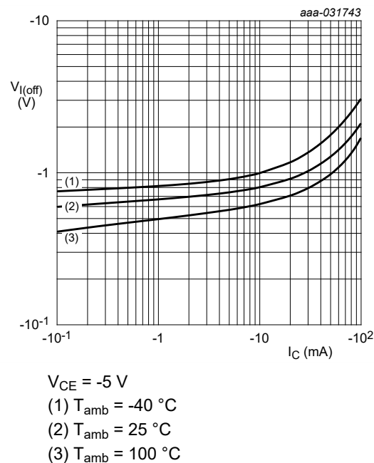
Fig. 7. NHDTA123JT-Q: Off-state input voltage as a function of collector current; typical values
