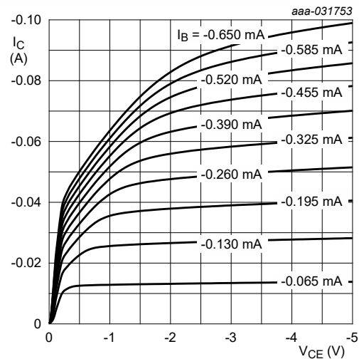
Fig. 17. NHDTA114YT-Q: Collector current as a function of collector-emitter voltage; typical values
