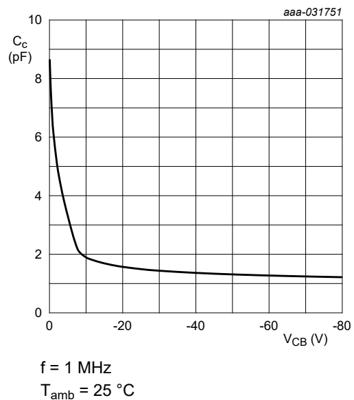
Fig. 15. NHDTA143ZT-Q: Collector capacitance as a function of collector-base voltage; typical values
